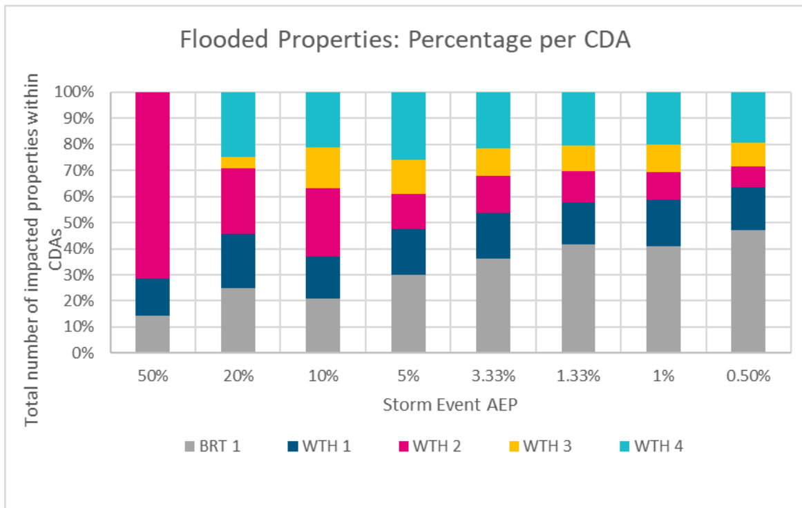
Figure 6-15 Percentage of Flooded Properties per Rainfall Event
