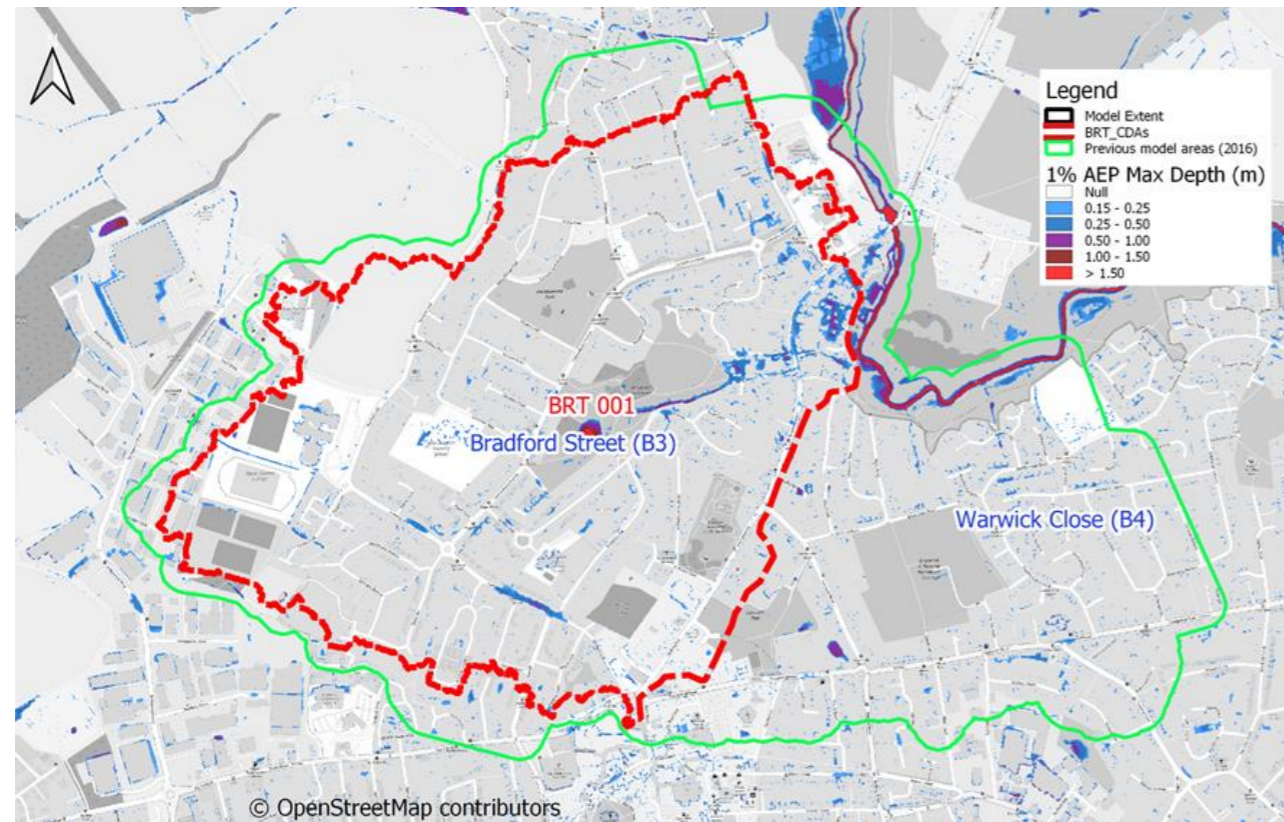
Figure 6-8 BRT 001 - 1% AEP Rainfall Event, Maximum Depth
