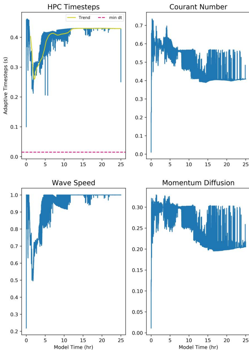
Figure F-1 1% AEP HPC stability
